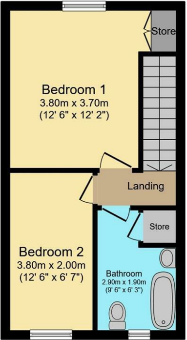
First Floor Floor area 30.8 sq.m. (331 sq.ft.)
